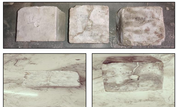
Fig. 8 Concrete blocks after self-healing
