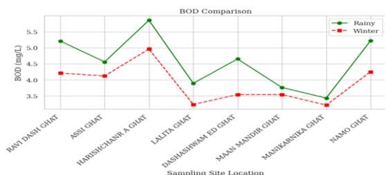
Fig.7 Biochemical Oxygen Demand (BOD) Levels at Varanasi Ghats
